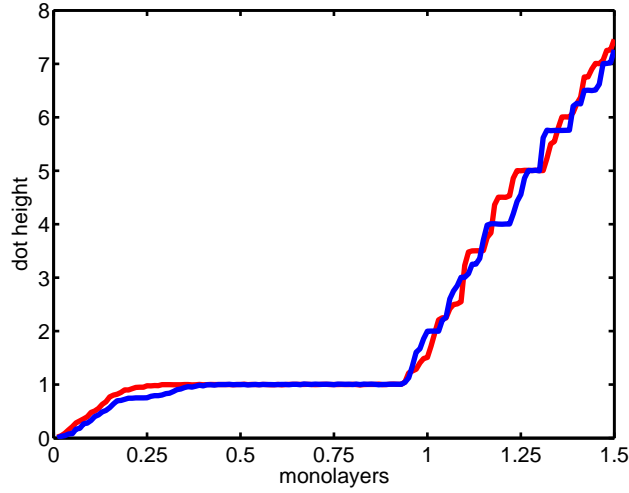
Figure 7: Dot height as a function of the number of deposited monolayers. The Surface Decomposition Method is plotted in blue, whereas the Local Energy Method is plotted in red. (color online)
