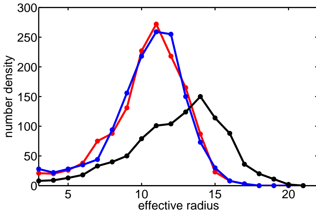
Figure 3: Island size distributions for the Local Energy Method (in red), Surface Decomposition Method (in blue), and with no elastic effects (in black). (color online)
