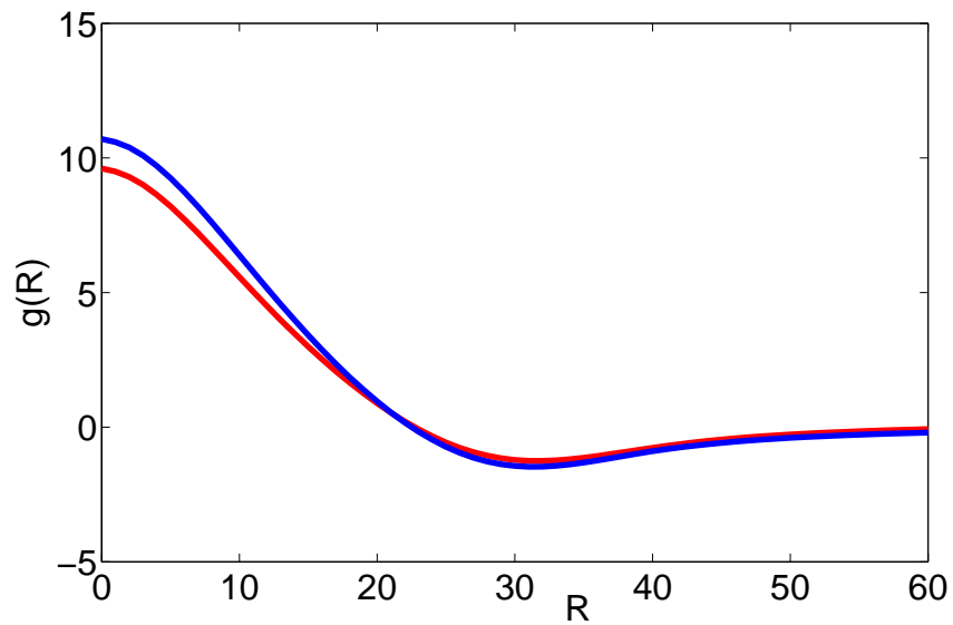
Figure 4: The red and blue curves are the ensemble averaged auto correlation function for the Surface Decomposition Method and the Local Energy Method, respectively. Ten simulations were used for each ensemble.
