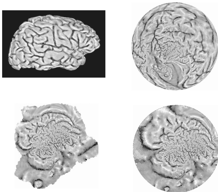
Figure 13. A 3D cortical hemisphere and three flat maps.
