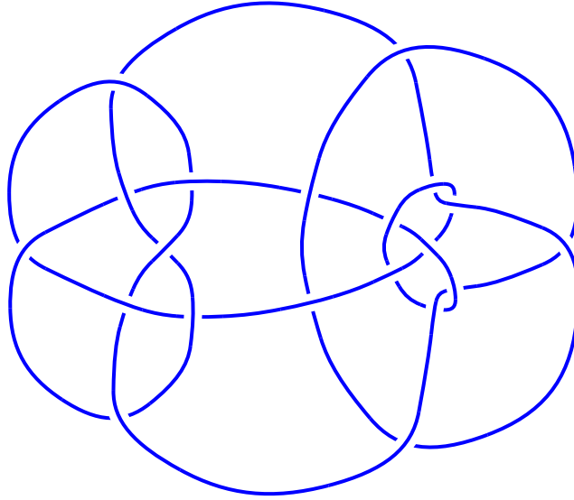
Figure 6: A 20-crossing satellite of the trefoil
