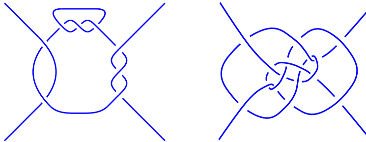
Figure 7: (i) A locally knotted tangle and (ii) a companion tangle
