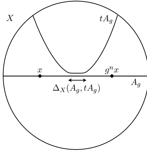
Figure 2: The small cancellation condition.
