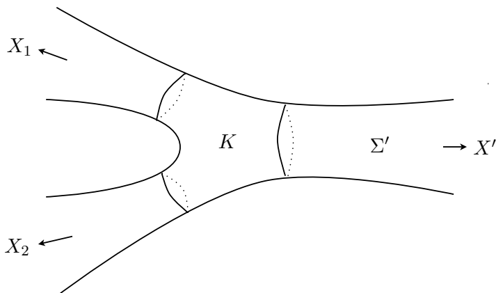
Figure 3: The situation in the third paragraph of the proof of Lemma 4.5.
